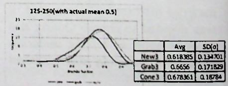
Figure 3: Normal distribution curves with standard deviation related to actual mean of sample (0.5) for particle size range 125-250µm
