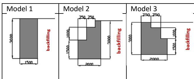
Fig. 1 Model dimensions
