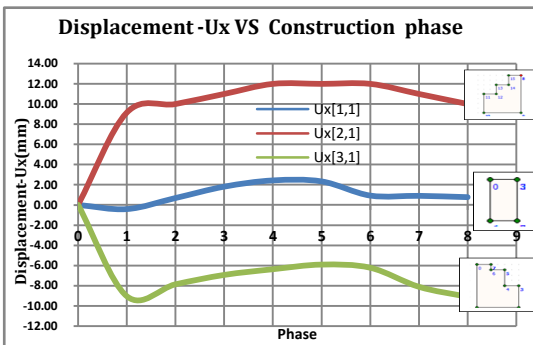
Fig. 2 Construction method 1 - (reference to top edge)
