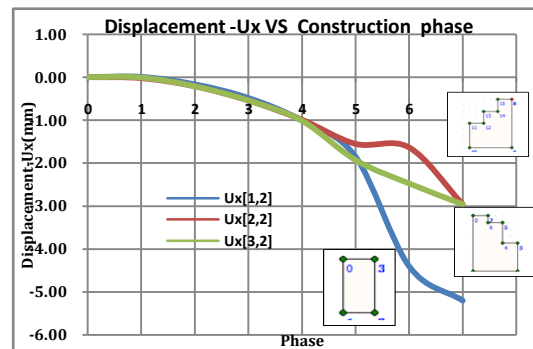
Fig. 5 Construction method 2 - (reference to bottom base)
