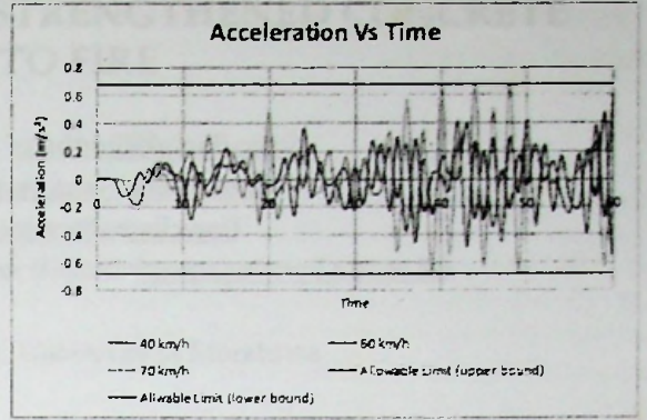
Figure 2 - Graphs for the Vertical Accelerations of Modified Bridge
