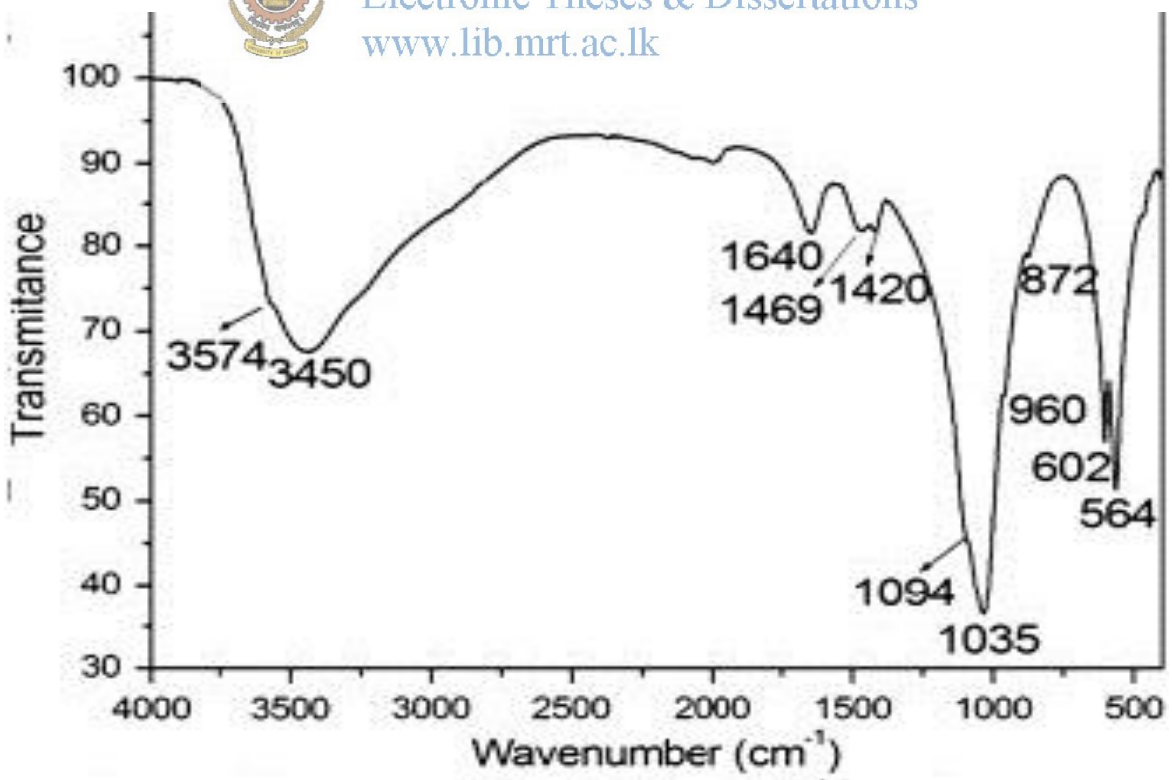
FT-IR spectrum of pure HA powder
