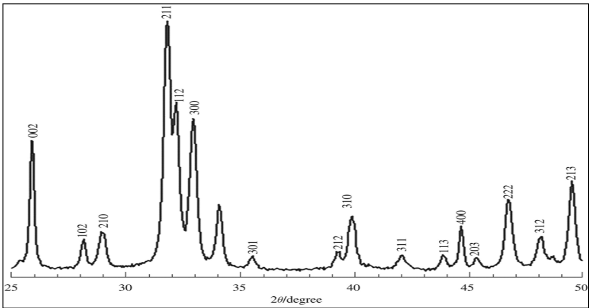
XRD spectrum of pure HA powder
