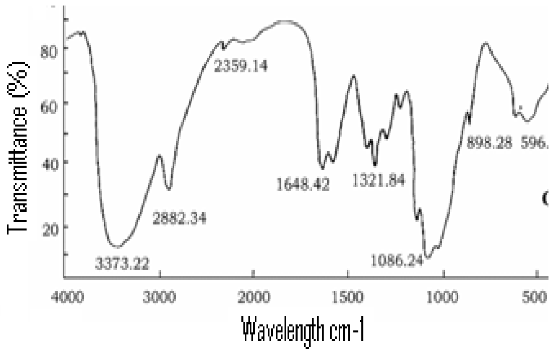
FT-IR spectrum of pure Chitosan
